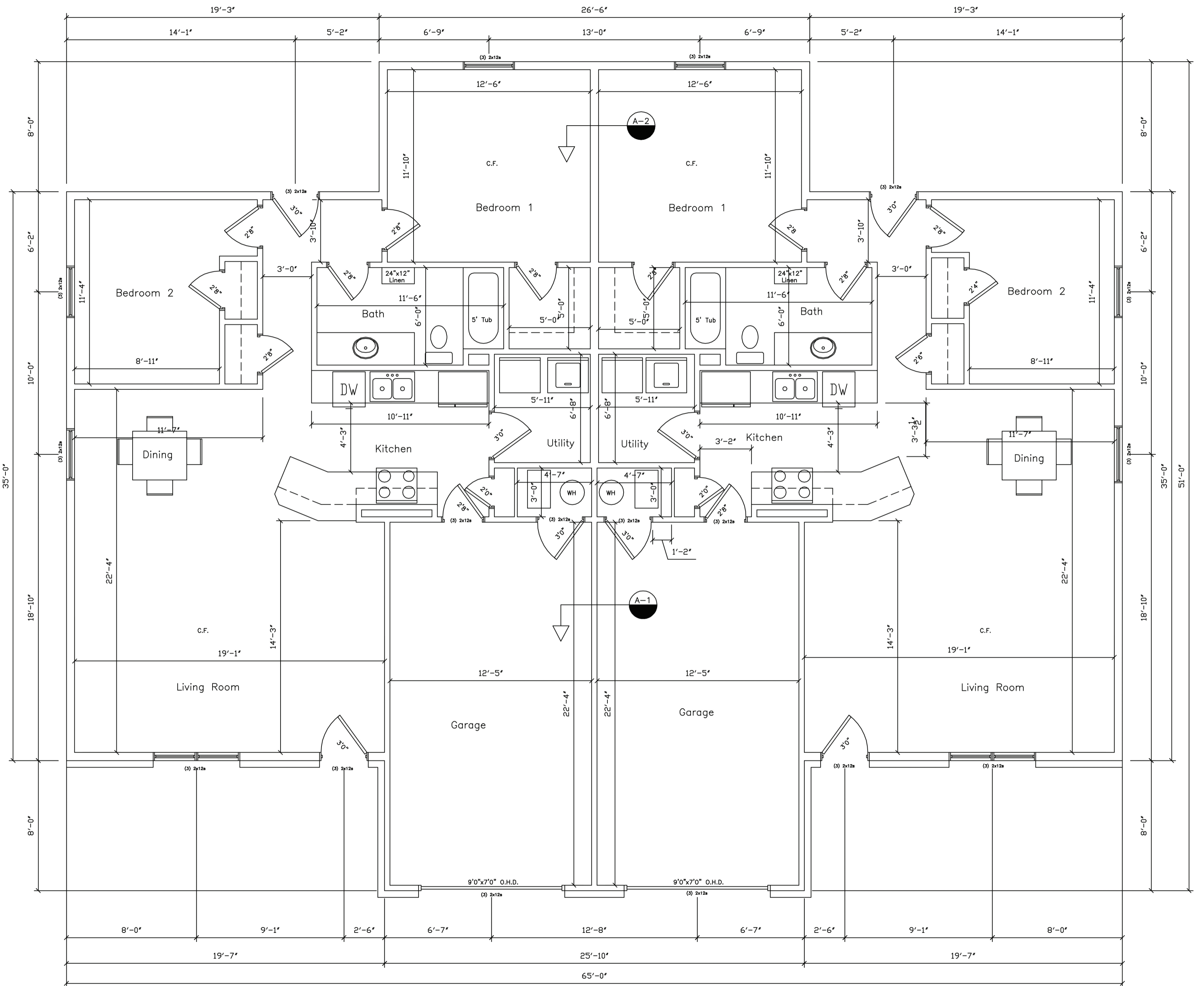
Floor Plan 1050 Sq. Ft. Per Unit 2x6-8' Walls
